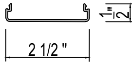
565-6501 Pillar Cap Profile
