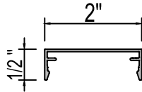
550-6201 Mullion Profile
